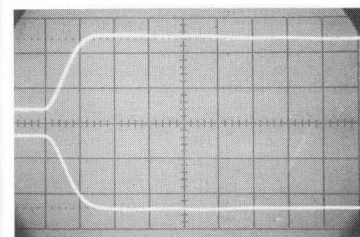
Fig. 4. Oscilloscope shows typical step response of new Power Amplifier driving 40-ohm load for both positive and negative 1-volt steps at input. Sweep speed: 0.1 \mu s/cm; vertical sensitivity: 5 V/cm.
